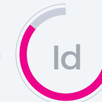
Indesign
